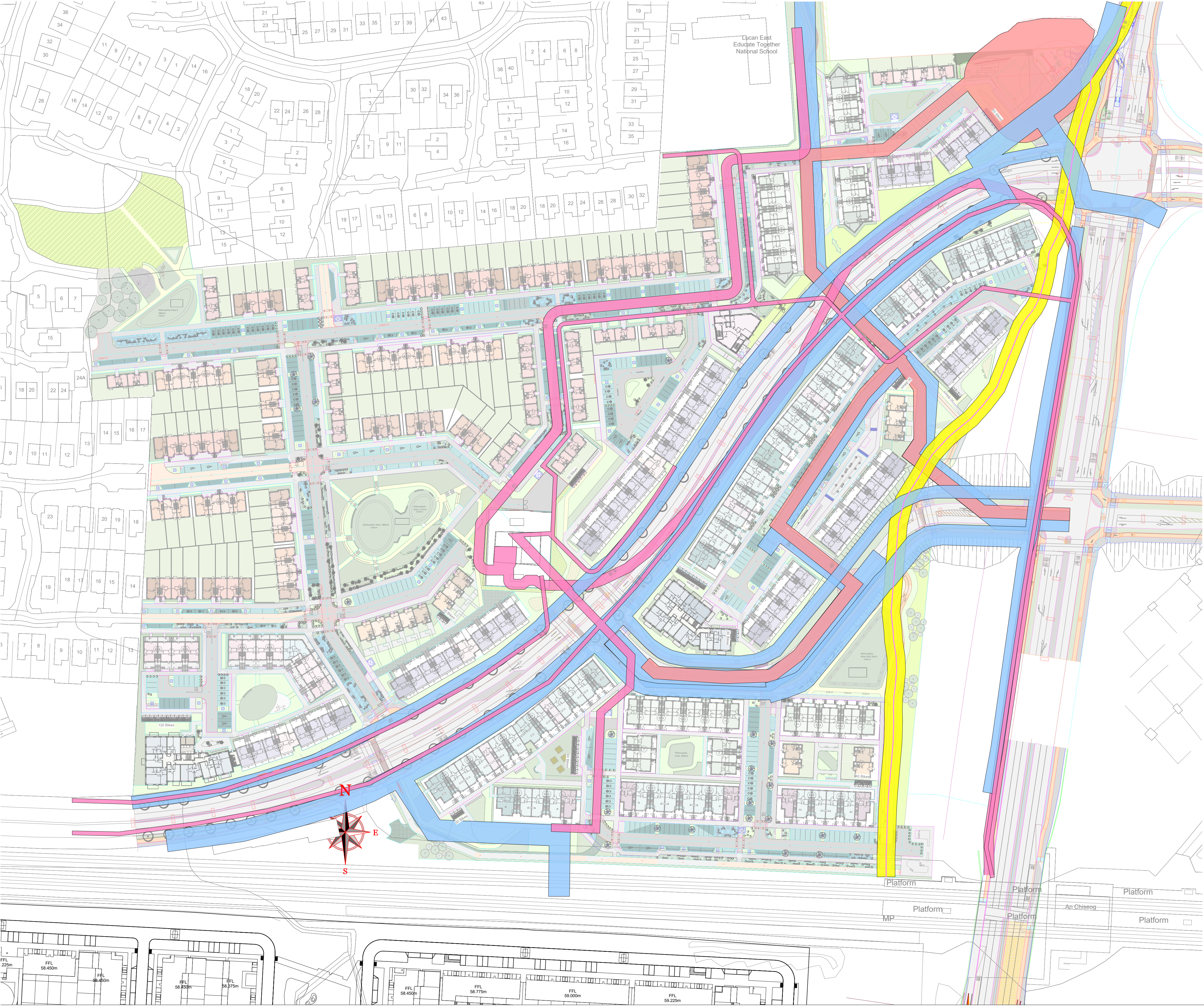
Site 3 Existing Realigned Services + Proposed Layout
